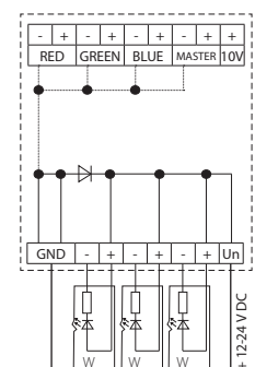
Monochrome LED strips control
