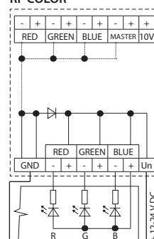
RGB LED strips control
